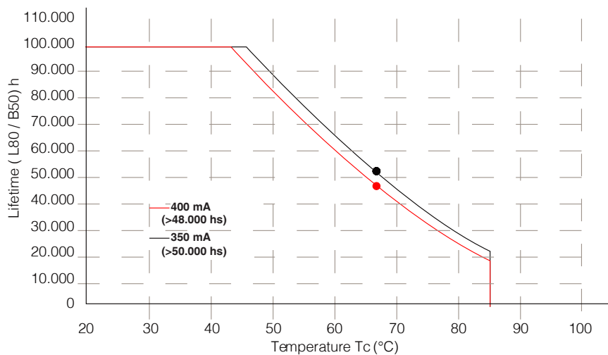
Lifetime Derating for MERAKI LINEAL MERAKI 702 ECO
